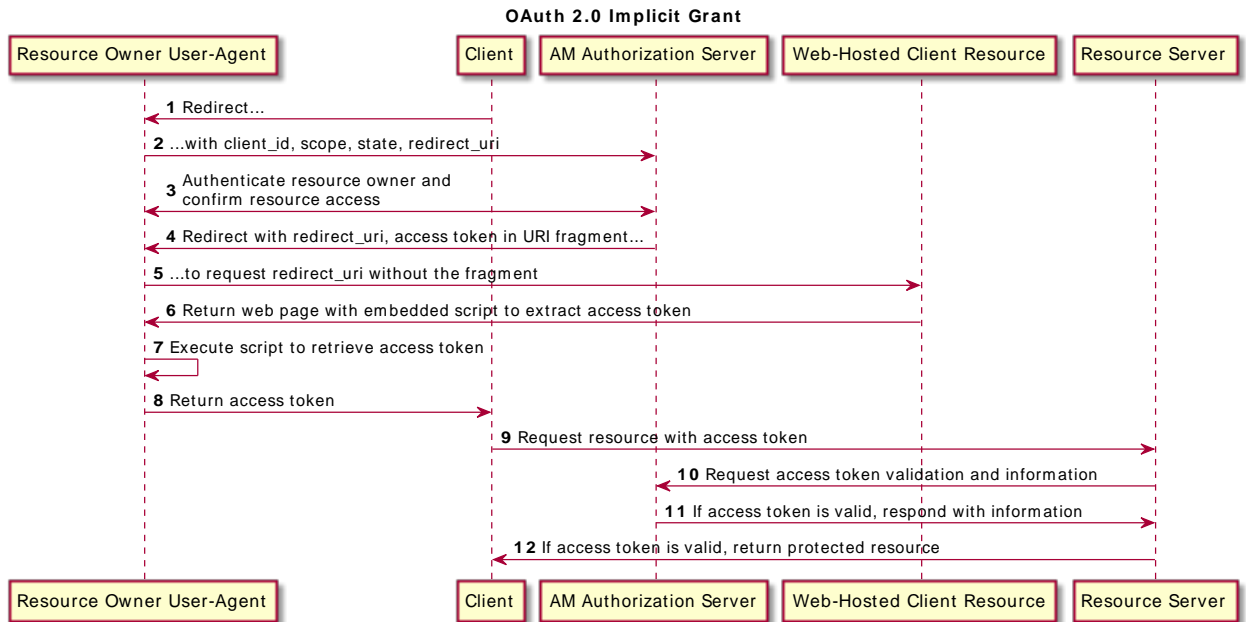
OAuth 2.0 Implicit Grant Process
