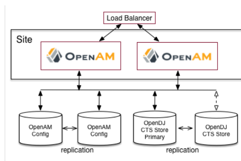
A Simple CTS Deployment
