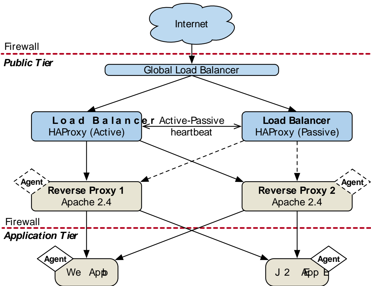
Frontend Load Balancers and Reverse Proxies with Agent
