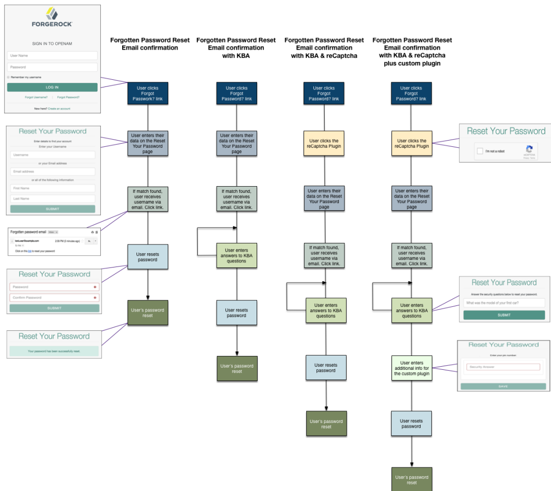
Forgotten Password Flow (Console)
