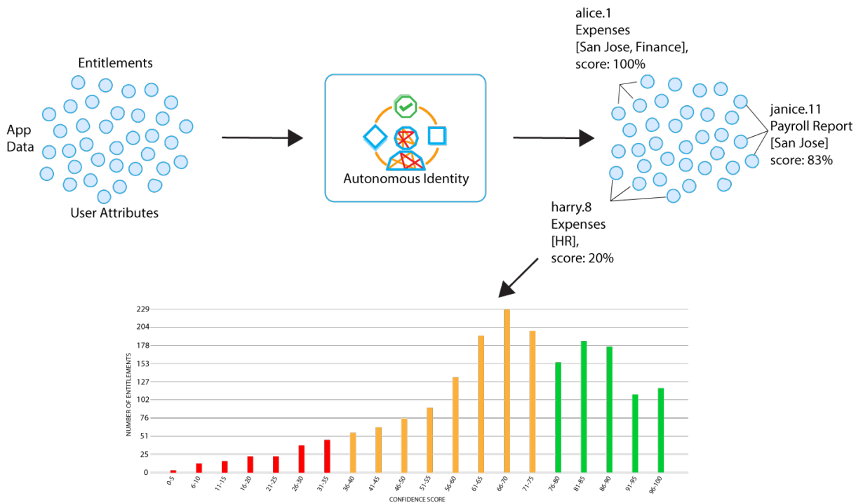
Figure 2: A simple conceptual diagram of Autonomous Identity
