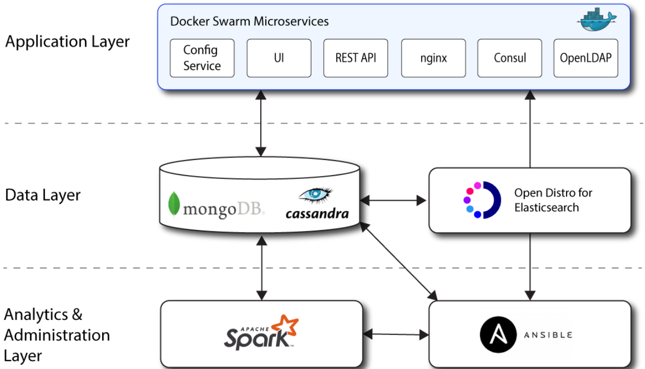
Figure 1: A Simple Conceptual Image of the Autonomous Identity Architecture
