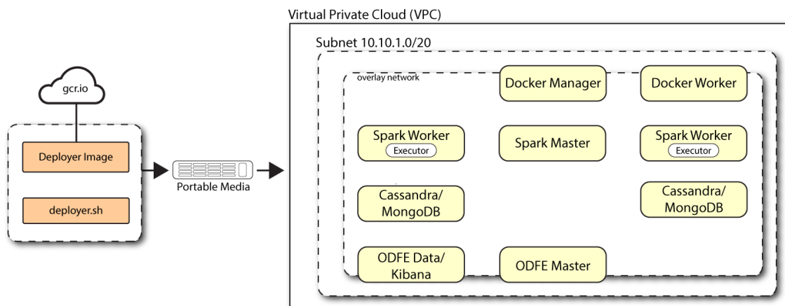
Figure 5: A multi-node air-gapped target deployment.
