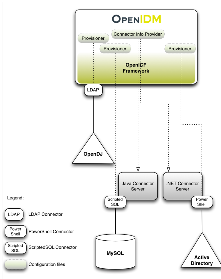
How IDM Uses the OpenICF Framework and Connectors
