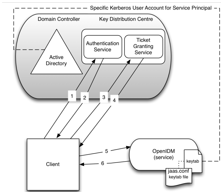
Client Authentication to IDM Using a Kerberos Ticket
