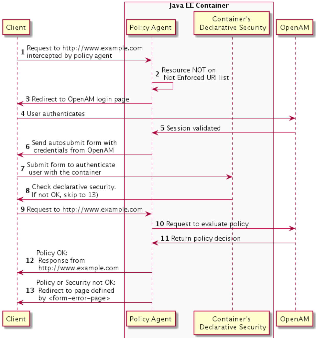
Figure 3.3. Declarative Security and Java EE Agent Flow
