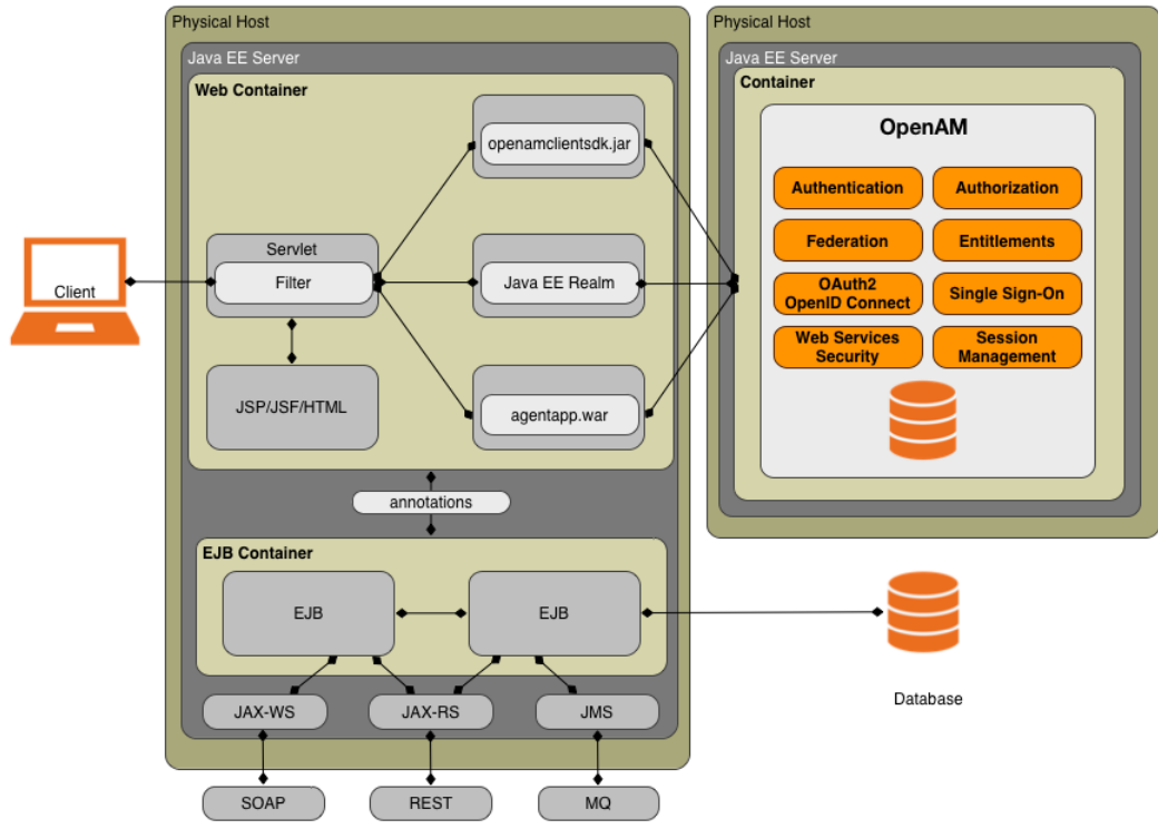
Figure 1.2. Java EE Policy Agent
