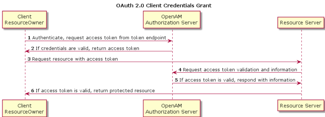
Figure 13.5. OpenAM in OAuth 2.0 Client Credentials Grant Process
