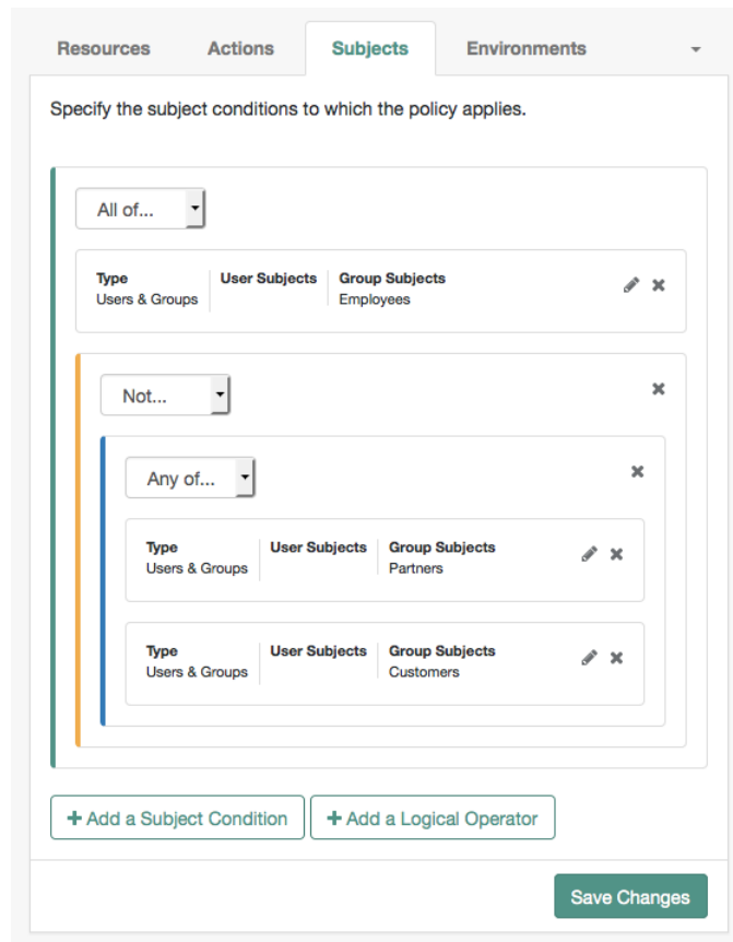
Figure 3.7. Nesting subject conditions
