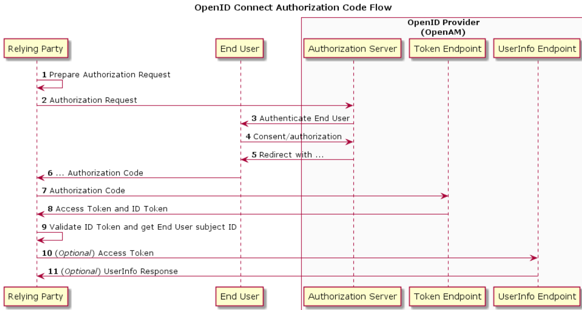
Figure 14.1. OpenAM in OpenID Connect Authorization Code Flow
