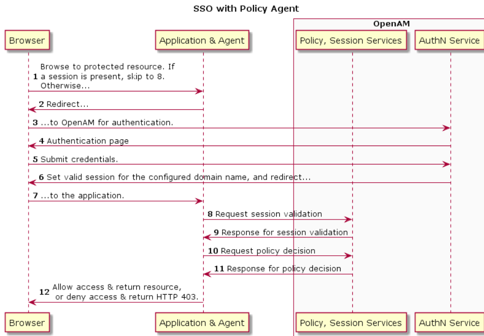
Figure 10.1. SSO With Policy Agent
