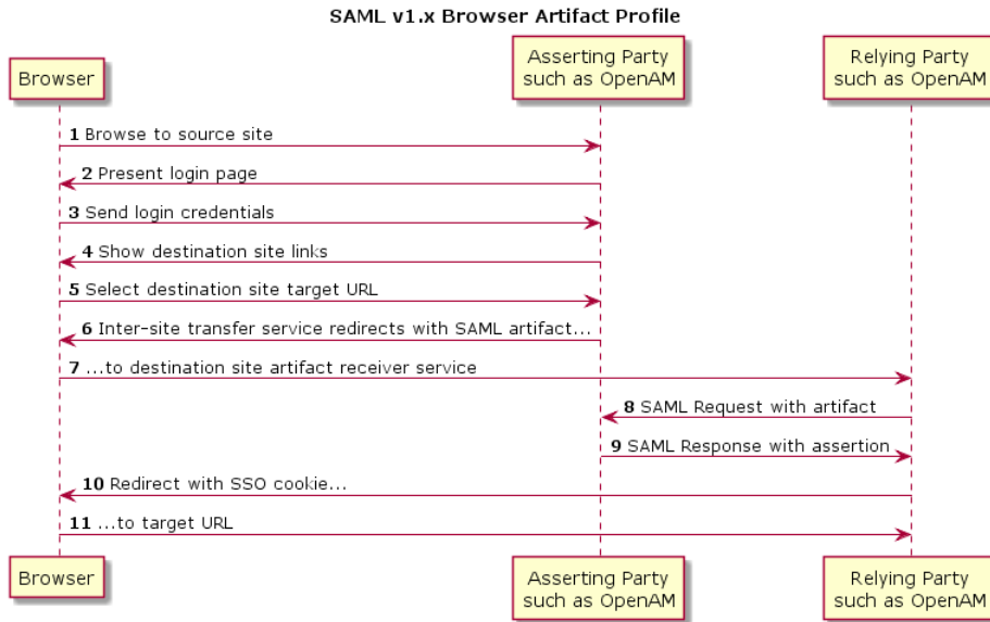
Figure 16.1. SAML v1.x Web SSO Browser Artifact Profile
