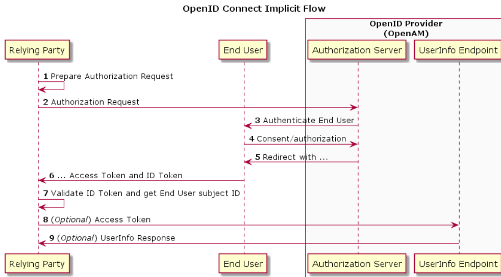
Figure 14.2. OpenAM in OpenID Connect Implicit Flow
