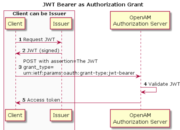
Figure 13.9. JWT Bearer as Authorization Grant
