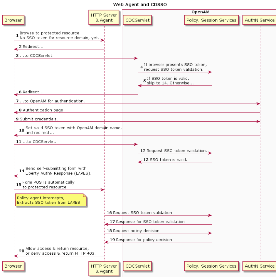
Figure 11.2. Web Policy Agent Mechanism for CDSSO
