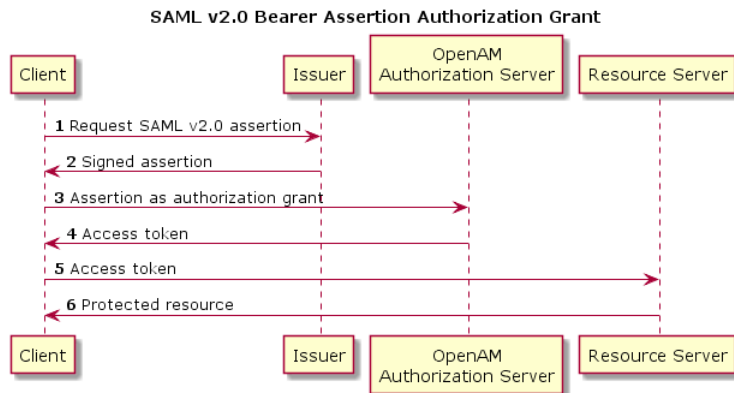
Figure 13.10. SAML v2.0 Bearer Assertion Authorization Grant
