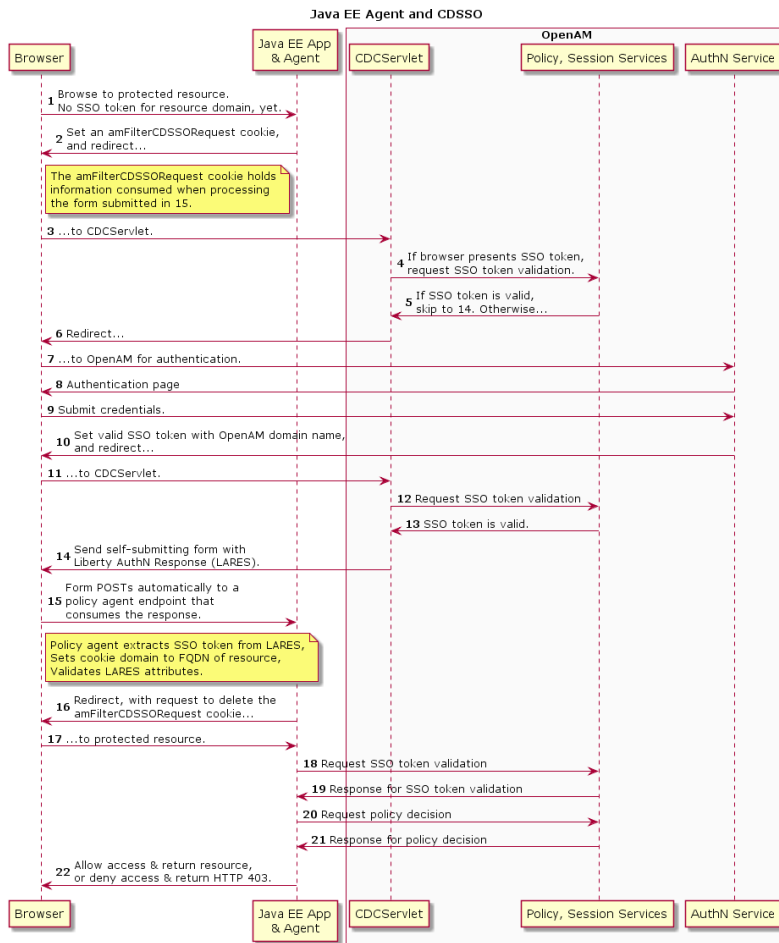
Figure 11.1. Java EE Policy Agent Mechanism for CDSSO
