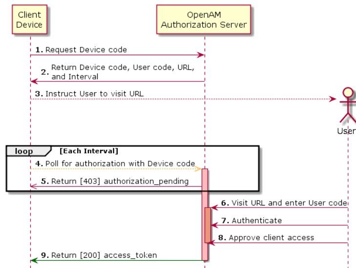
Figure 13.6. OAuth 2.0 Device Flow
