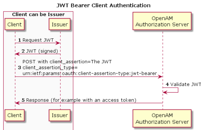
Figure 13.8. JWT Bearer Client Authentication
