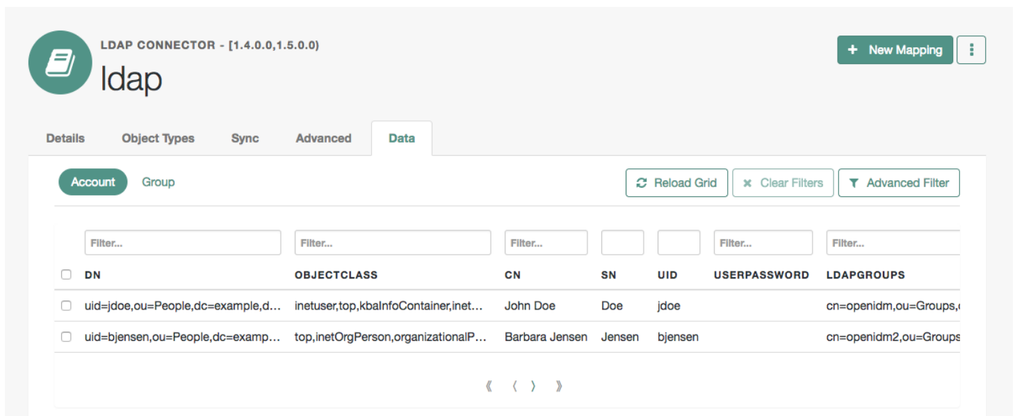
Figure 1. Data Tab For a Connected LDAP Resource
