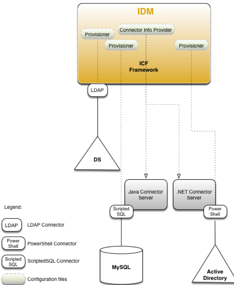
Figure 1. How IDM Uses the ICF Framework and Connectors
