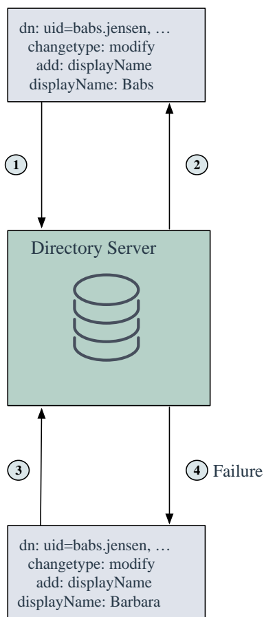
Conflicting Operations in Standalone versus Replicated Environments
