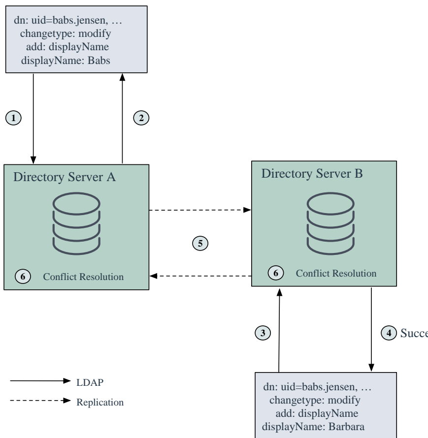
Conflicting Operations in Standalone versus Replicated Environments
