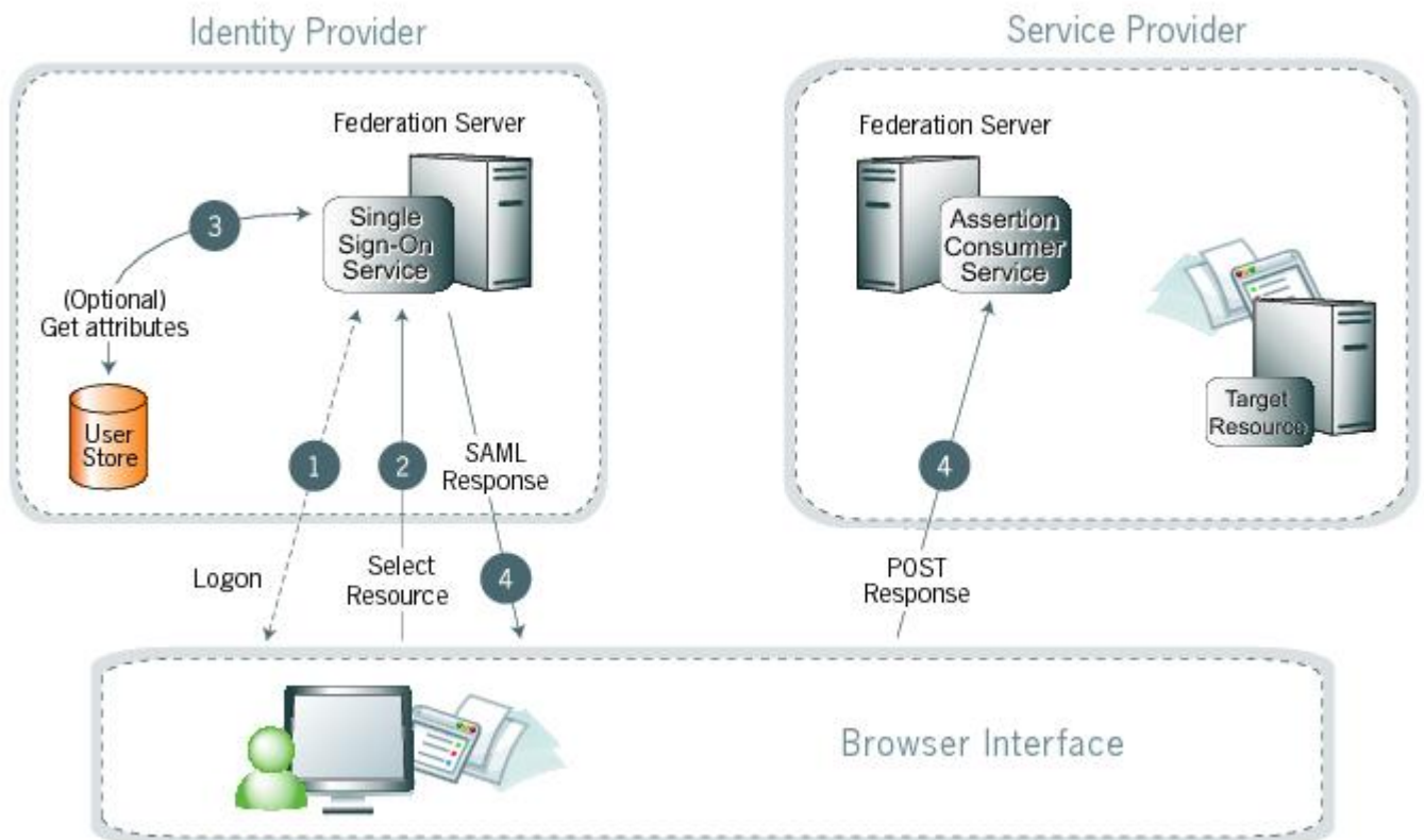
Figure 2: Browser/POST Profile
