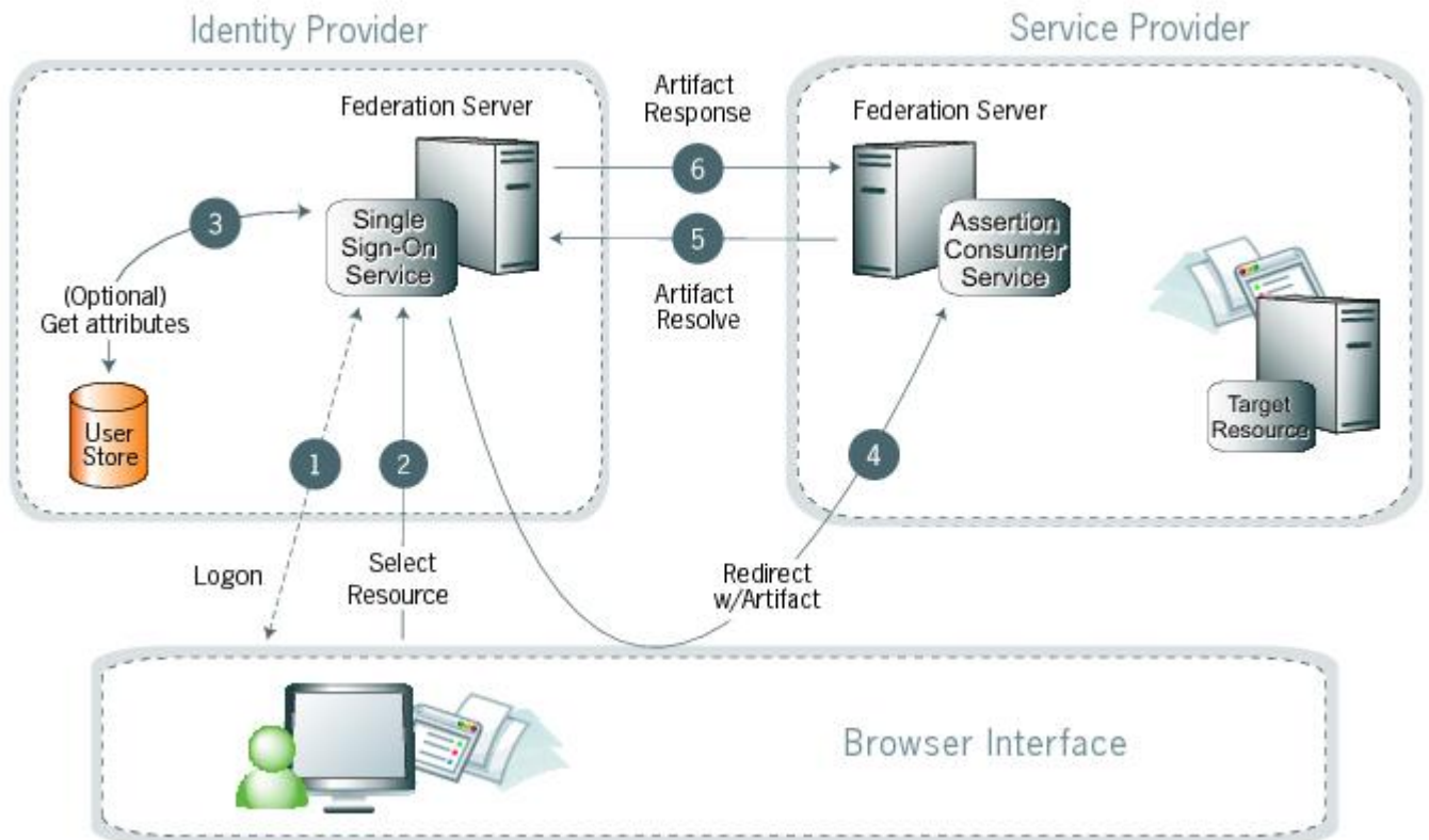
Figure 3: SSO:Browser/Artifact Profile
