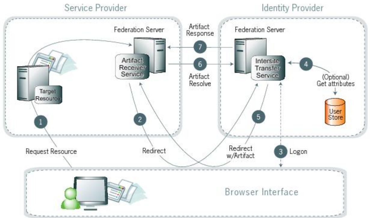
Figure 5: SP-initiated SSO
