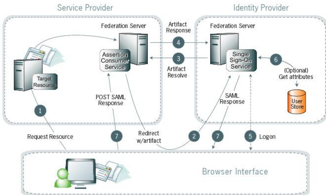
Figure 8: SP-initiated SSO: artifact/POST
