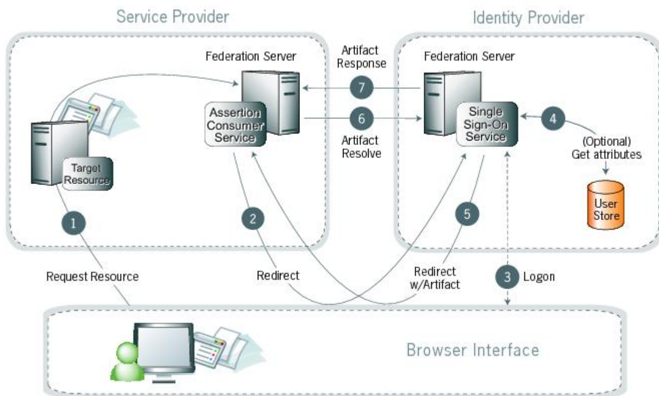
Figure 10: SP-initiated SSO: redirect/artifact
