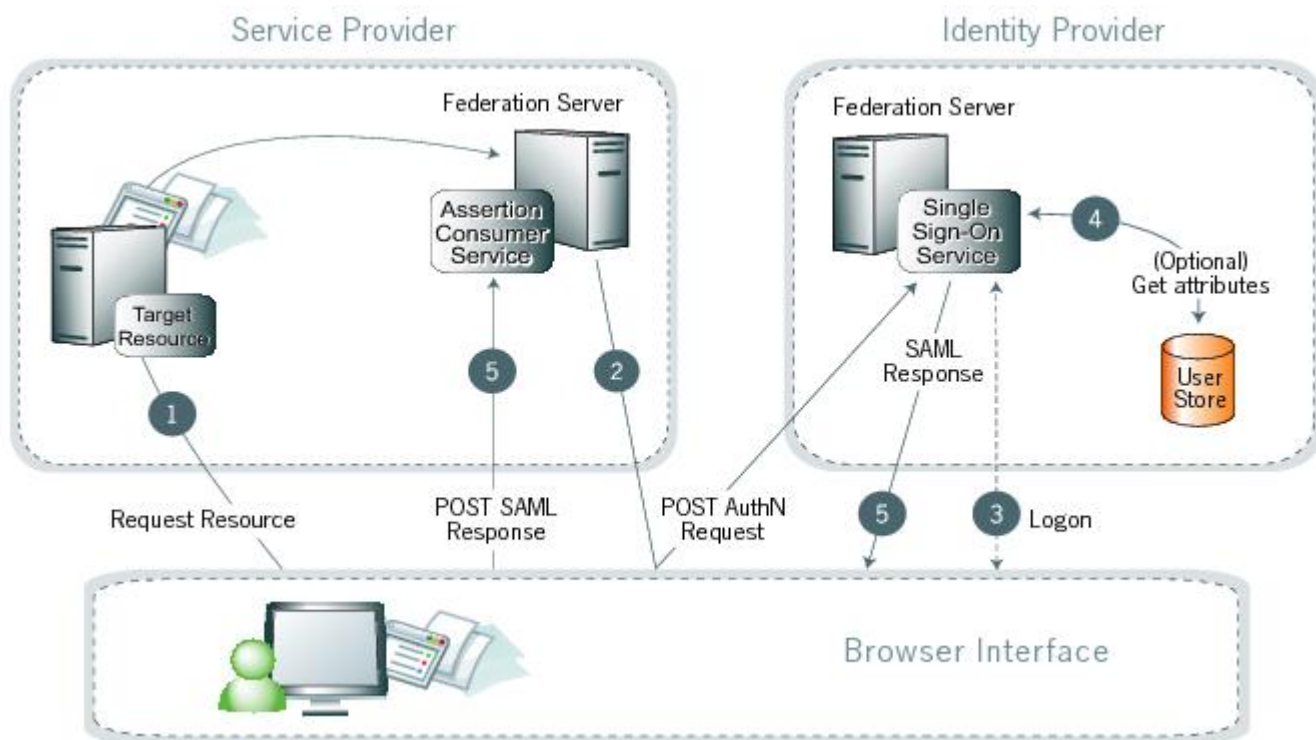
Figure 6: SP-initiated SSO: POST/POST
