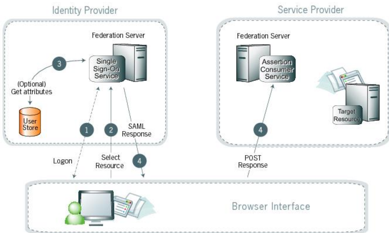
Figure 12: IdP-initiated SSO: POST
