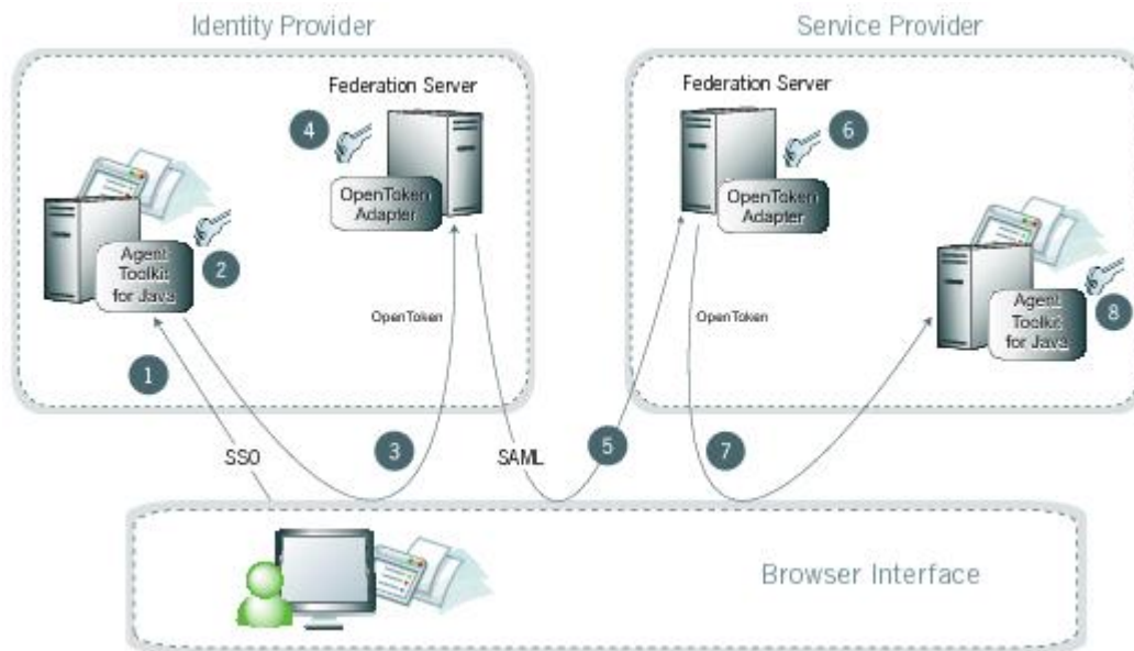
Figure 24: SP-Initiated SSO: POST/POST
