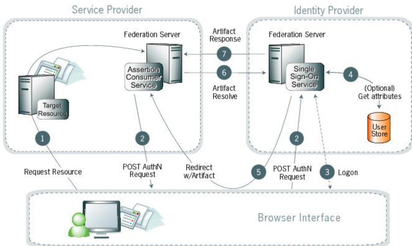
Figure 9: SP-initiated SSO: POST/artifact
