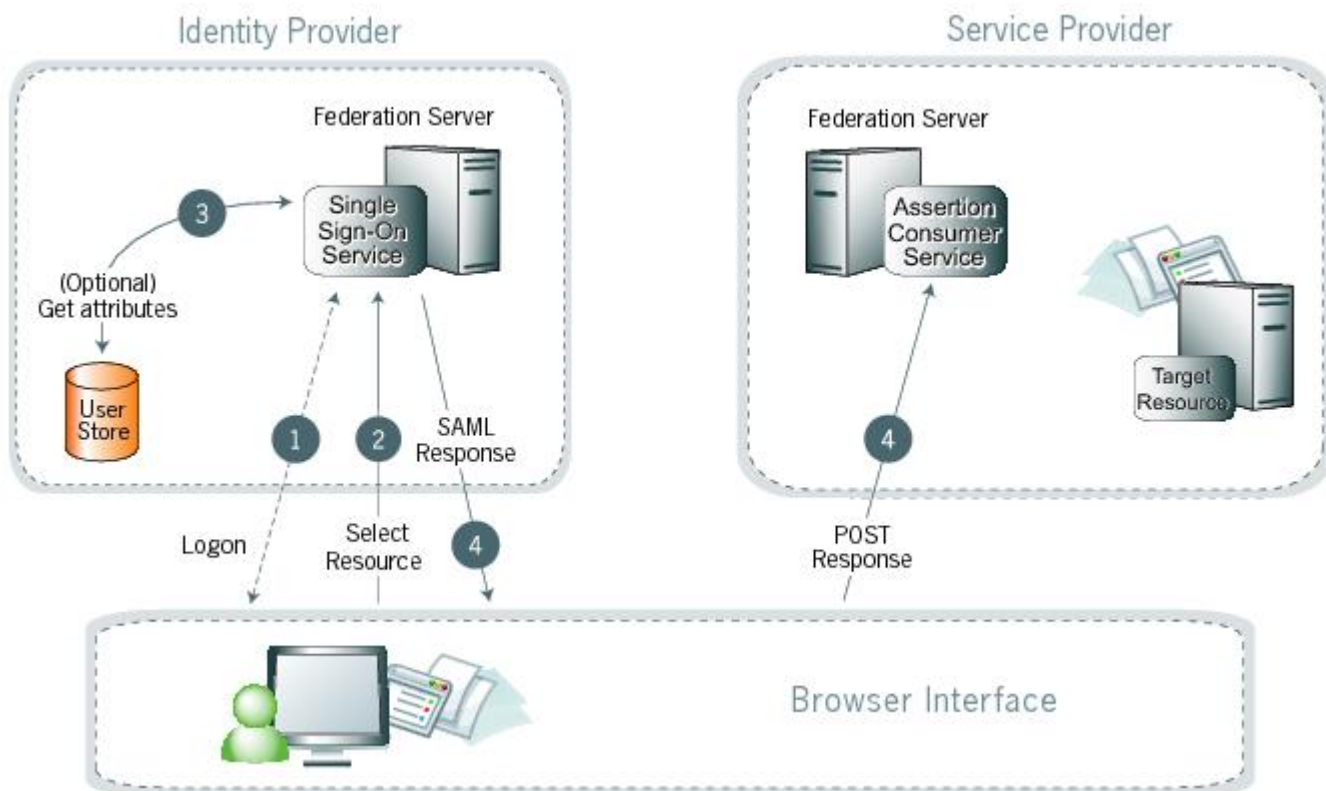
Figure 3: SSO browser/POST profile
