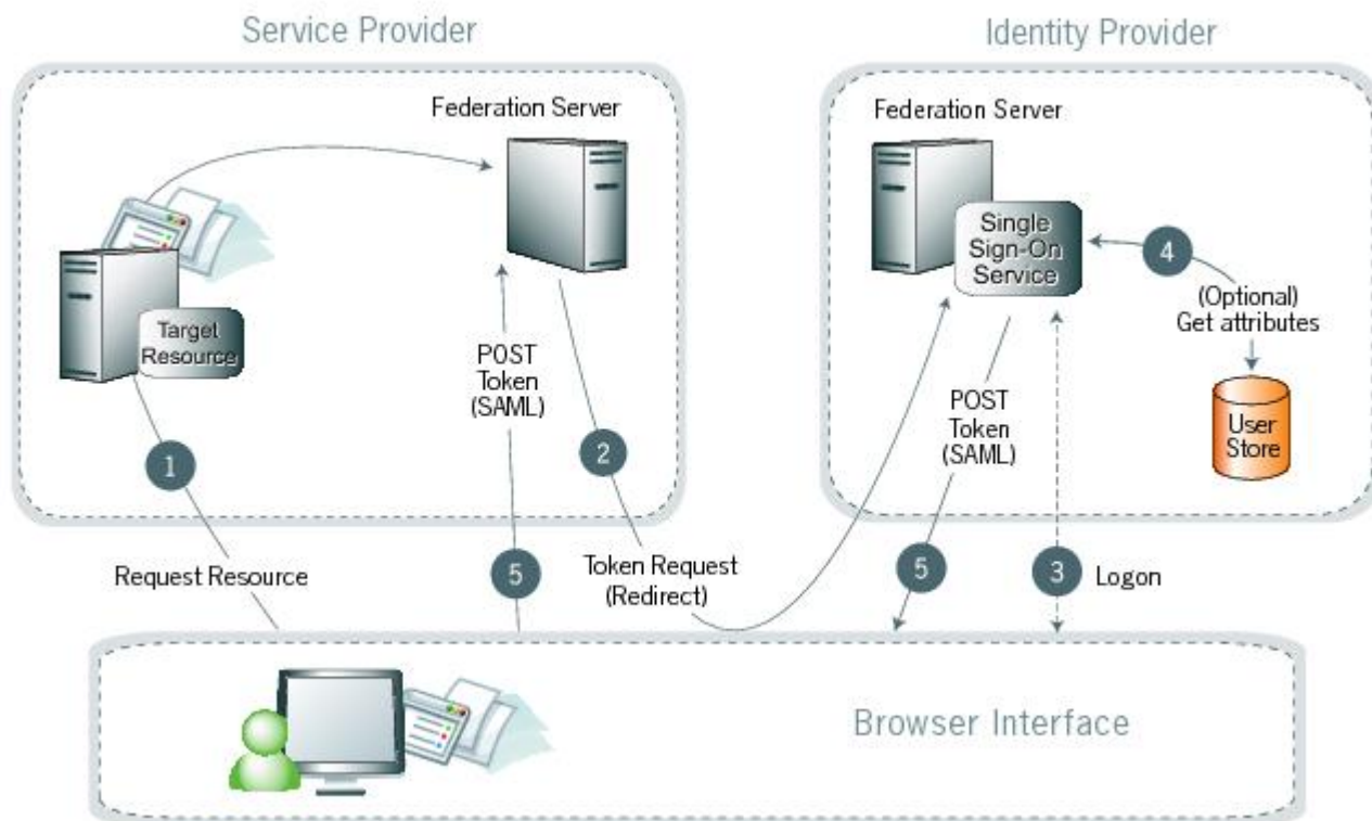
Figure 14: WS-Federation SSO
