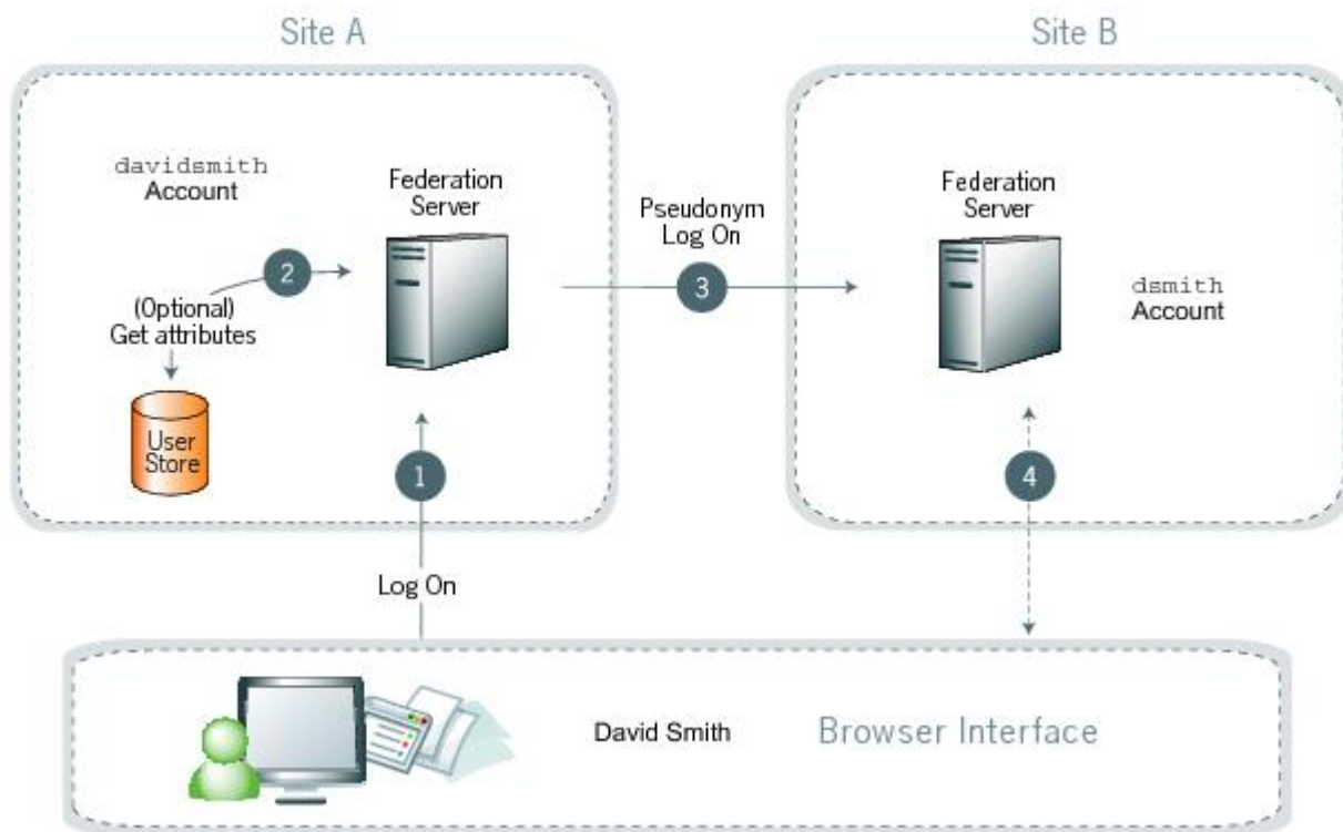
Figure 15: Account linking
