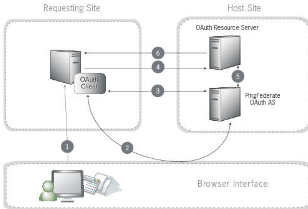
Figure 18: Web redirect flow
