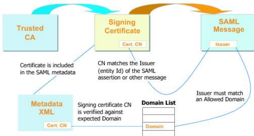
Figure 21: Auto-Connect Security Model
