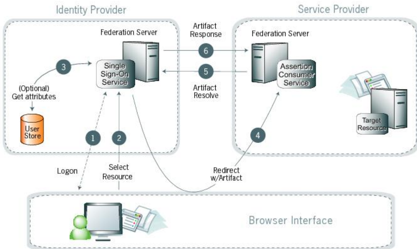
Figure 4: SSO browser/artifact profile
