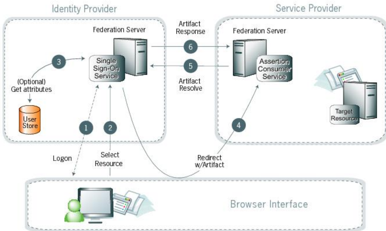
Figure 13: IdP-initiated SSO: artifact
