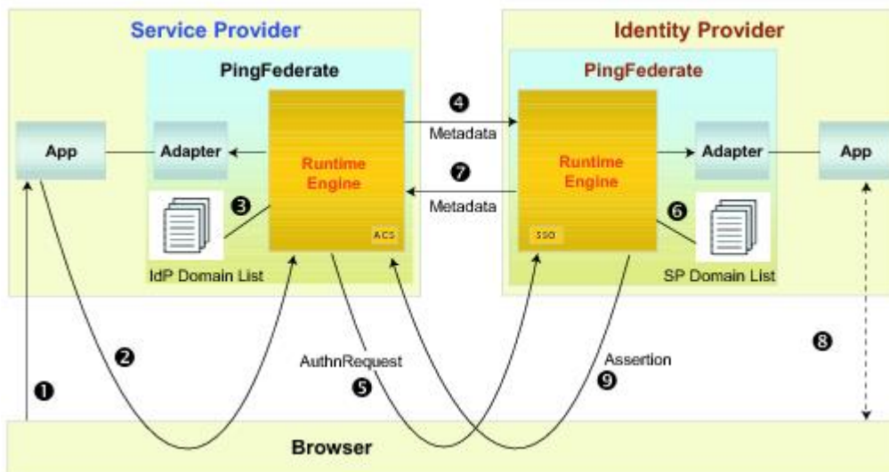
Figure 20: Auto-Connect Processing Flow
