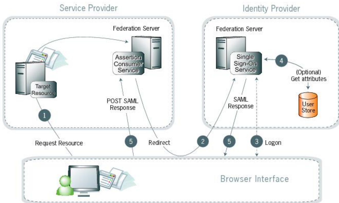
Figure 7: SP-initiated SSO: redirect/POST
