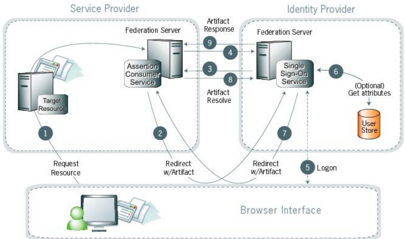
Figure 11: SP-initiated SSO: artifact/artifact
