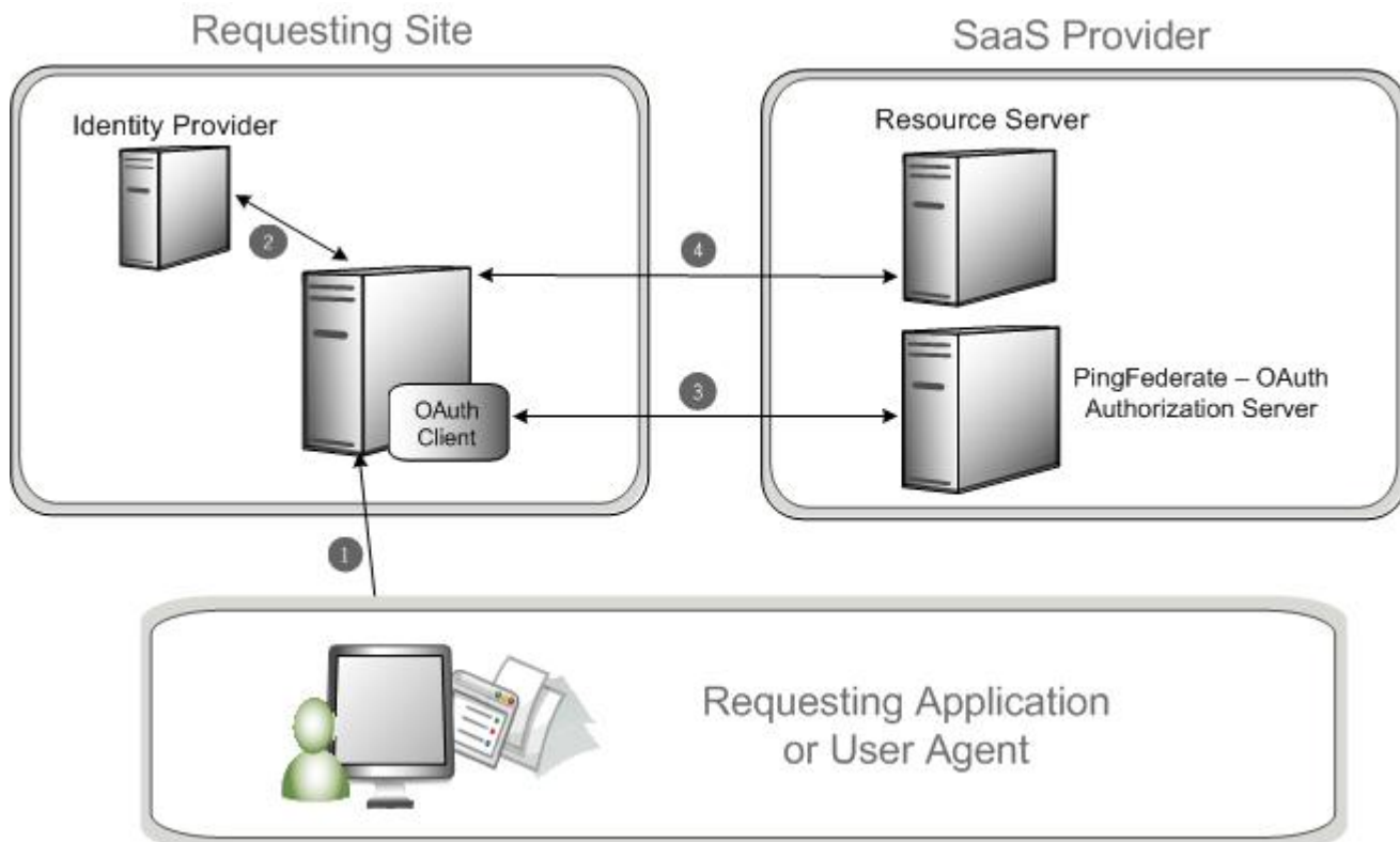
Figure 19: Assertion grant profile
