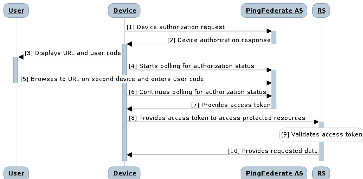
Figure 19: OAuth device flow
