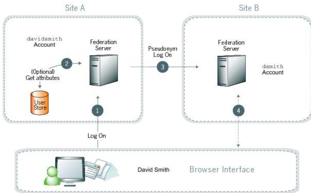
Figure 15: Account linking
