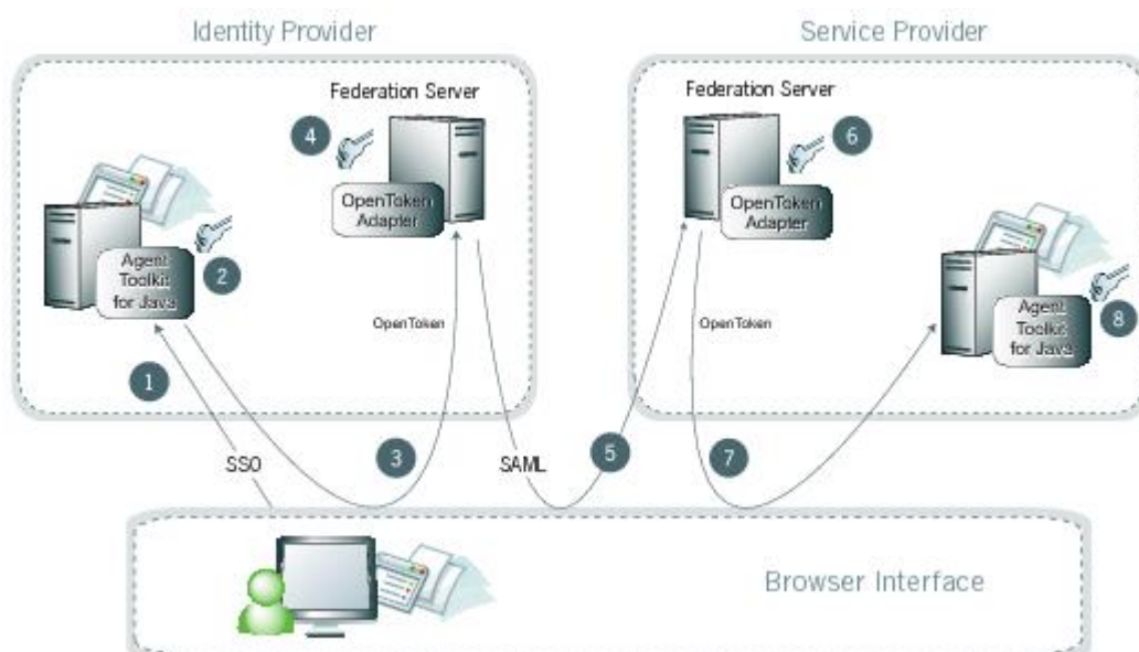
Figure 23: IdP-Initiated SSO: POST/POST
