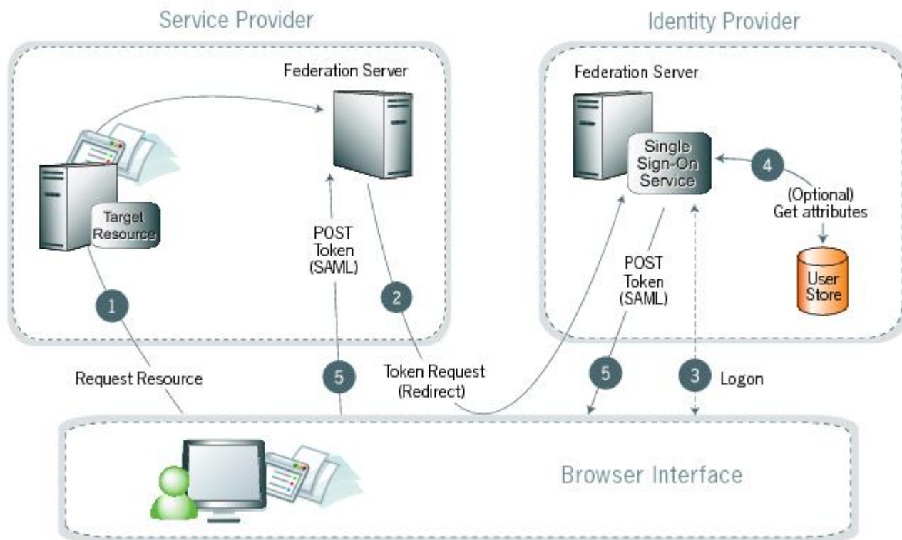
Figure 14: WS-Federation SSO
