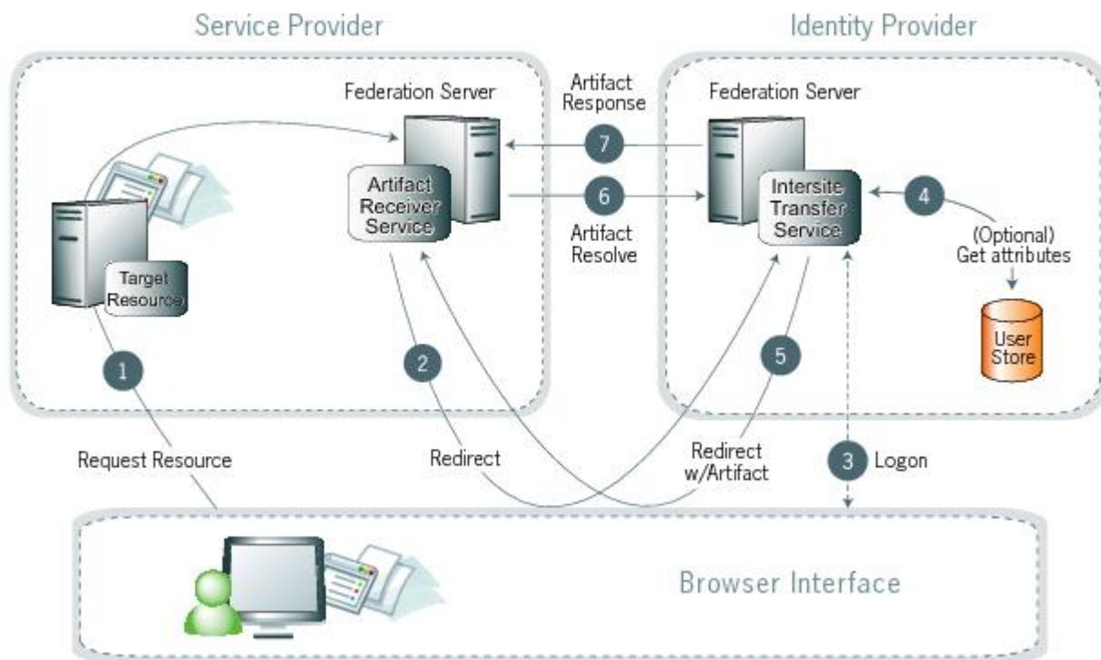
Figure 5: SP-initiated SSO
