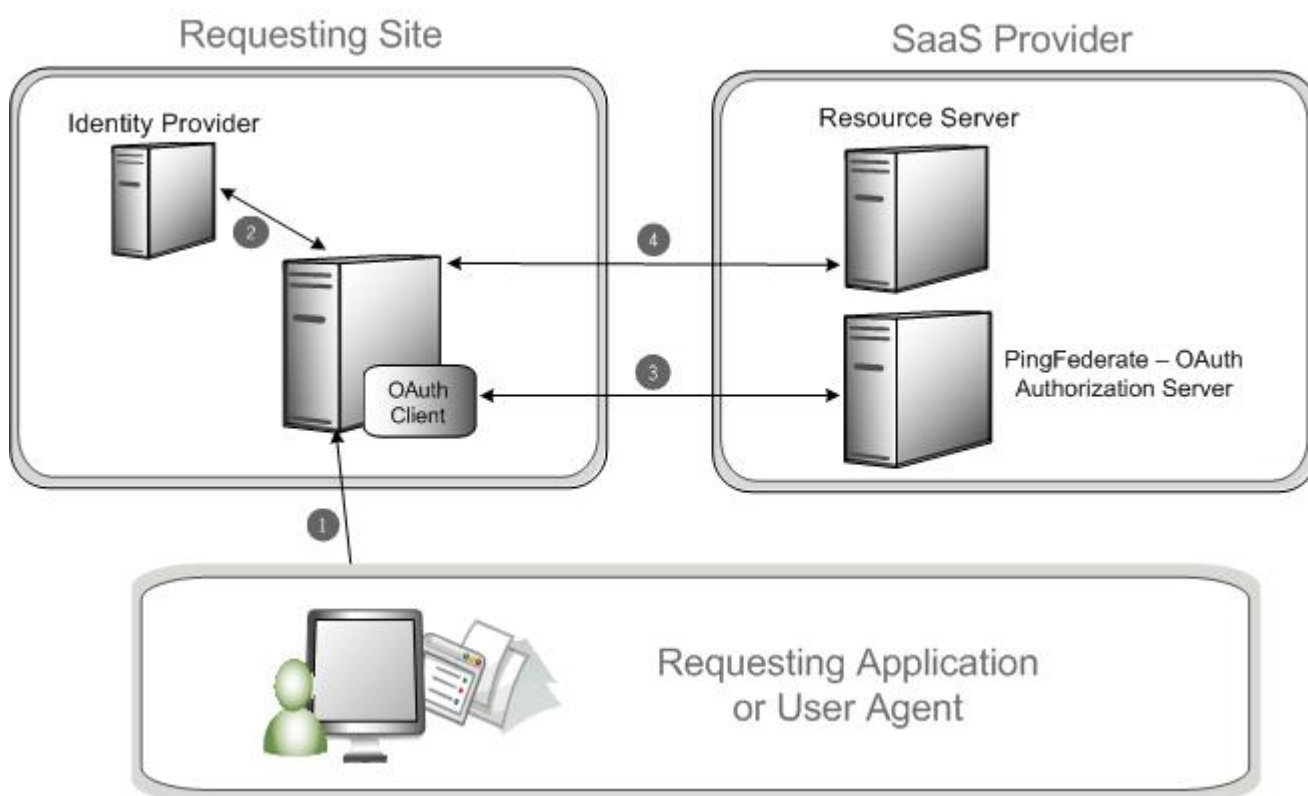
Figure 20: Assertion grant profile
