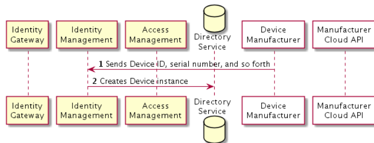
Figure 2.1. Creating and Storing a Device Identity
