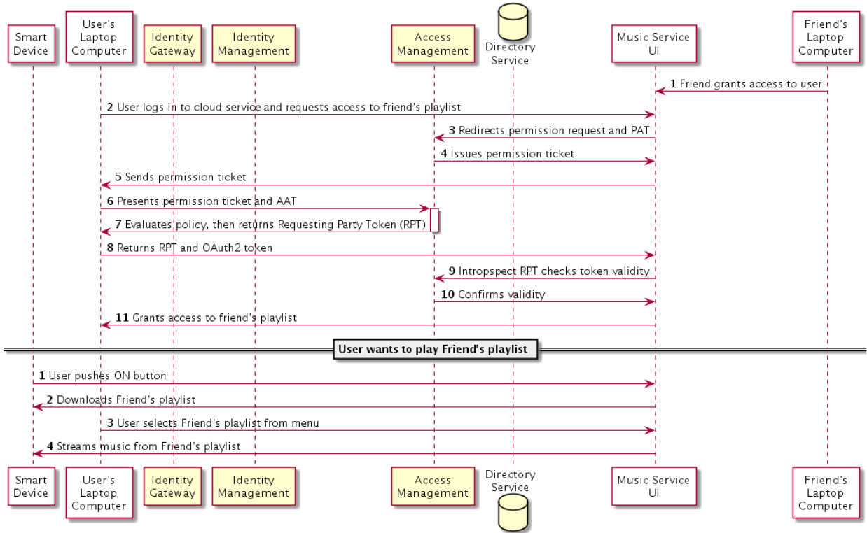
Figure 2.5. User-Managed Access
